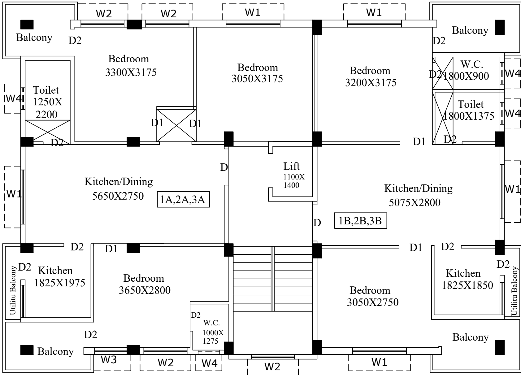
1ST, 2ND & 3RD FLOOR PLAN
